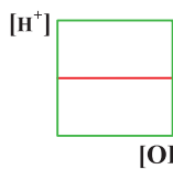
[\text{OH}^-]
